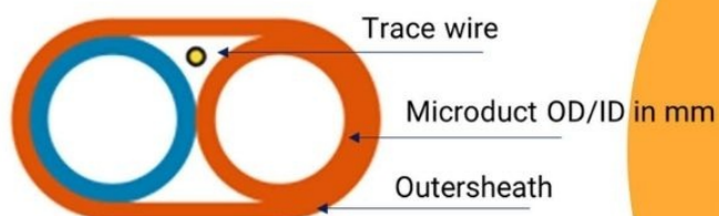
Number of Microduct – 2 tubes ( 2way)
