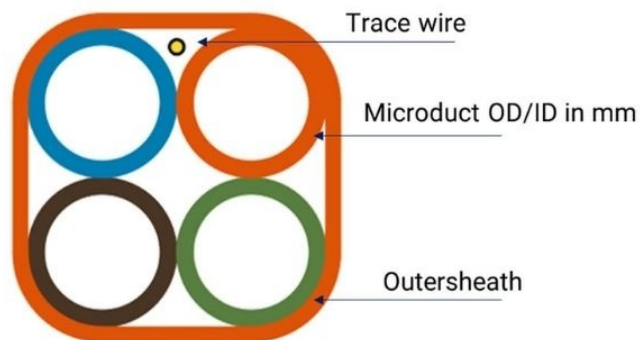
Number of Microduct – 4 tubes ( 4way)
